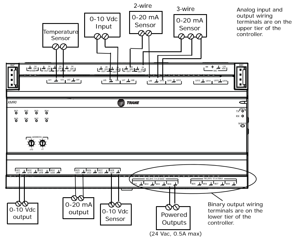
Figure 4. XM90 input and output wiring examples
