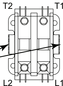
Double Pole Contactor (MS)*
